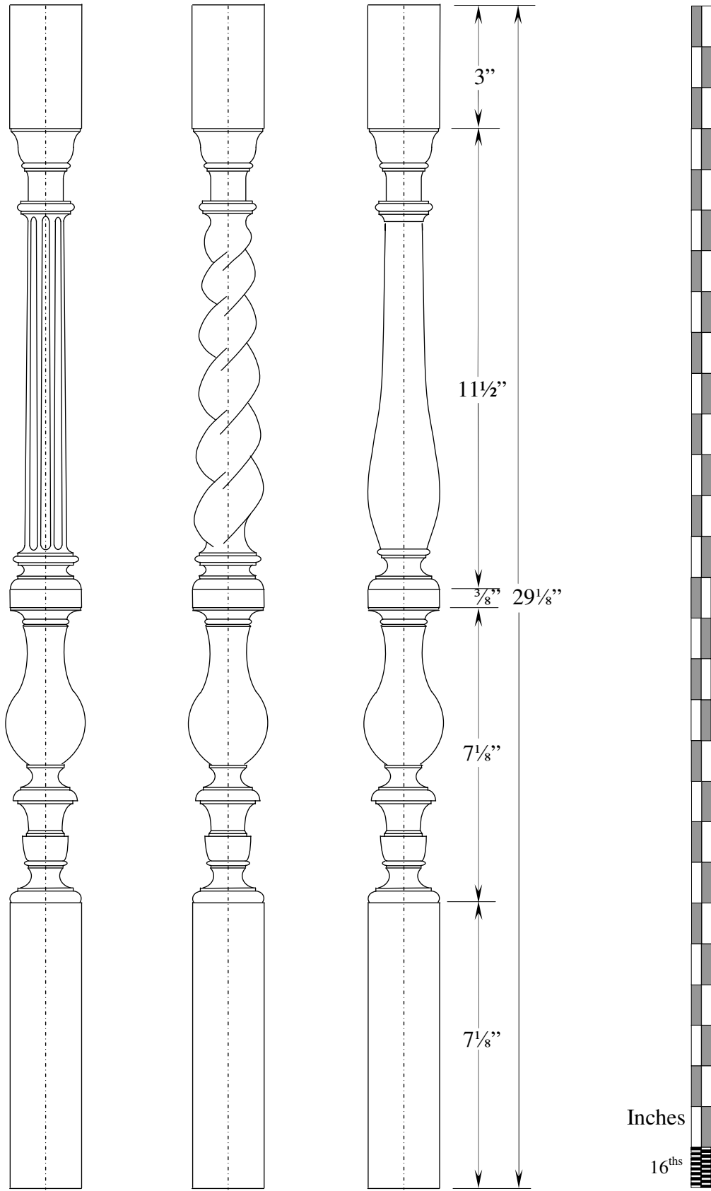
PISCATAQUA TYPE BALUSTERS
