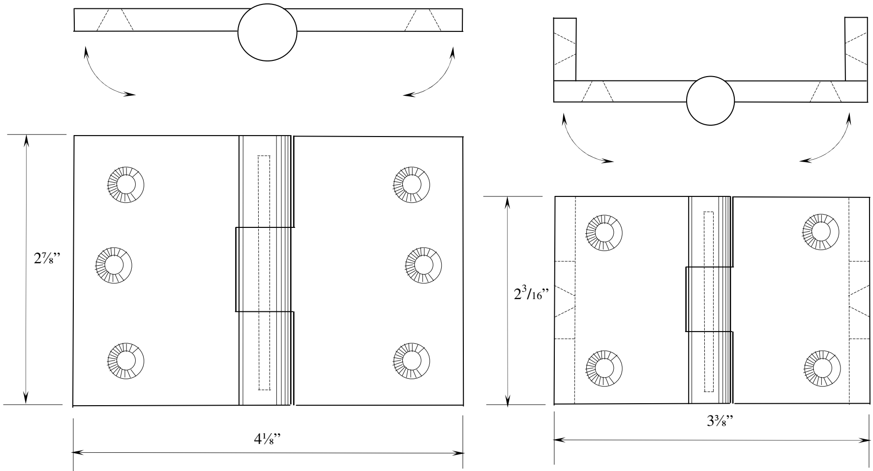
Butts for Pew Doors
