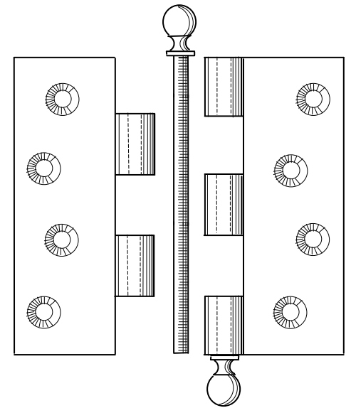
Slip Pin Butt
