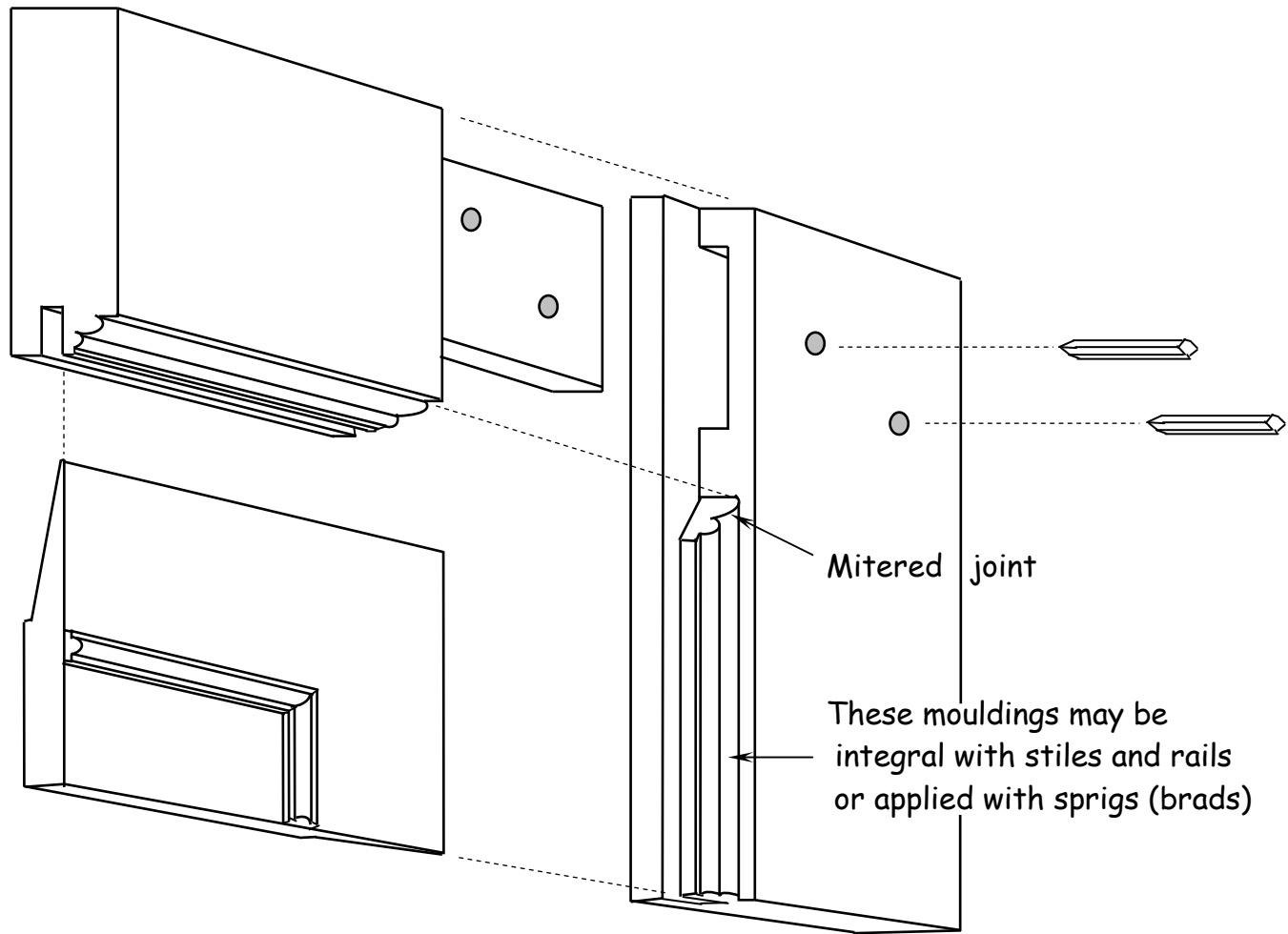
FEDERAL STYLE DOOR, EXPLODED VIEW
