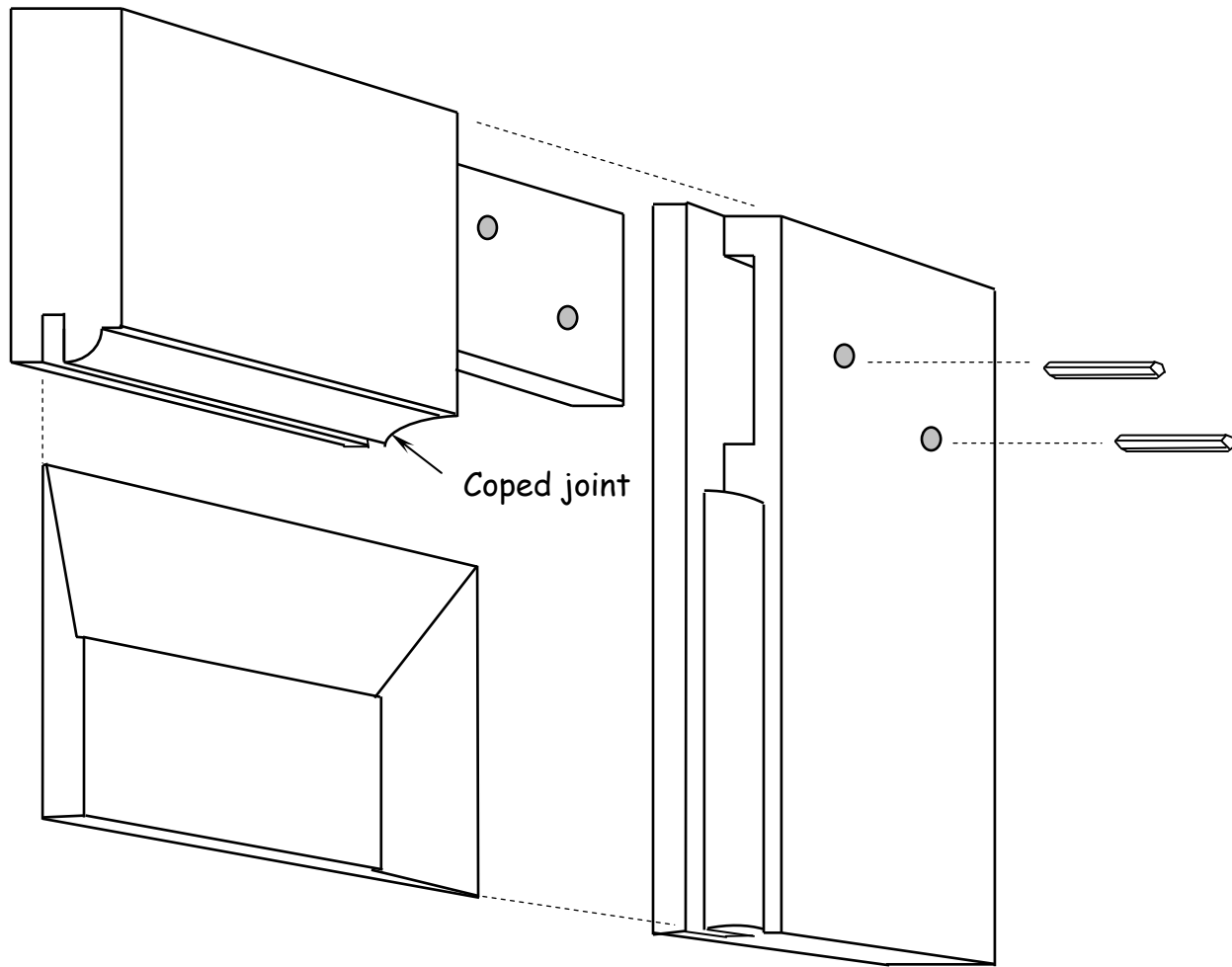
GEORGIAN STYLE DOOR, EXPLODED VIEW
