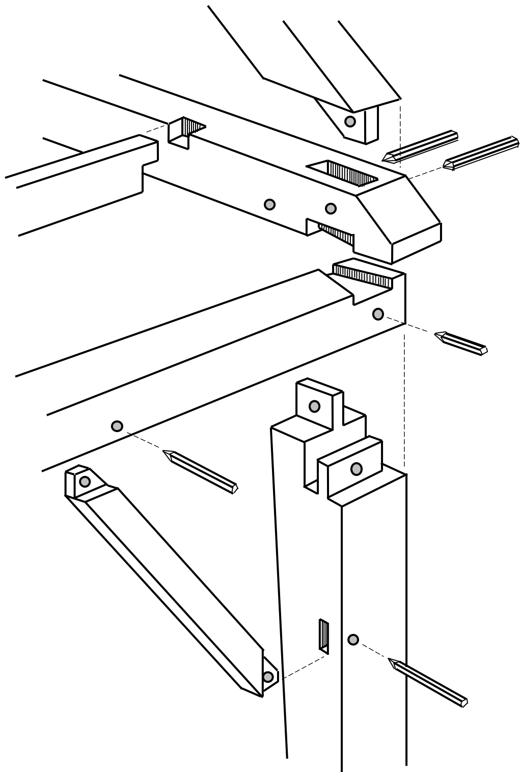
Exploded Scribe Rule Joints: typical 18 th -century corner post, wall plate, tie beam, rafter, attic floor joist, and wall brace.
