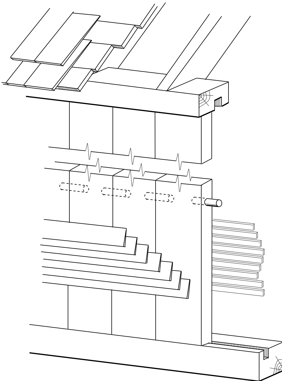
Alternative method of attaching bottoms of wall planks
