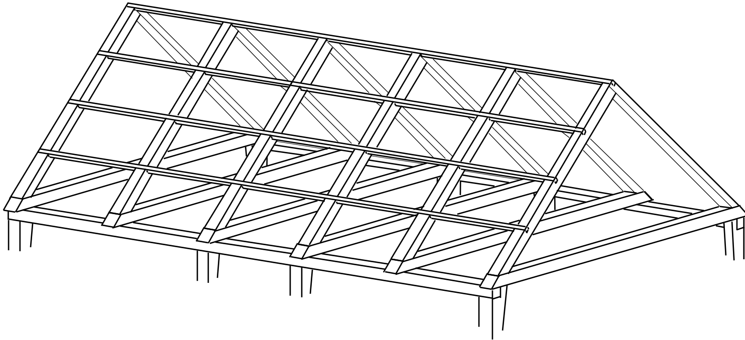
Rafter and Purlin Roof Frame
