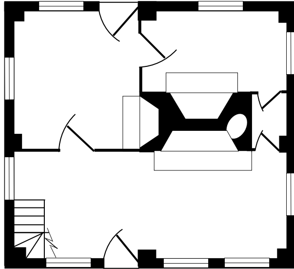
Square plan dwelling
