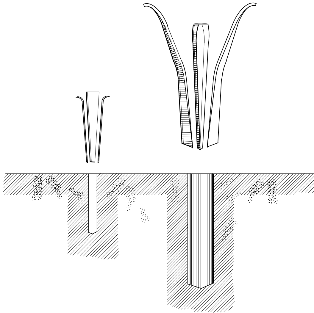
Flat Wedge in Slot
